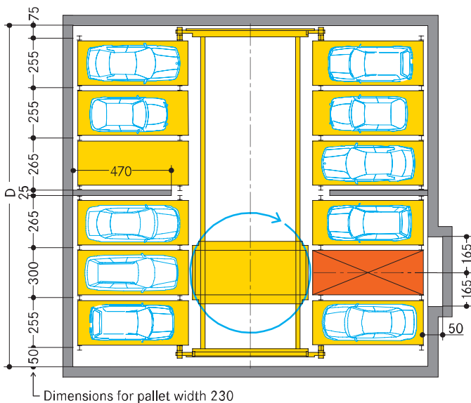
Dimensions for pallet width 230
